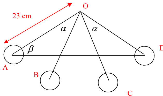
Fig. 2: Layout of the sorting station
